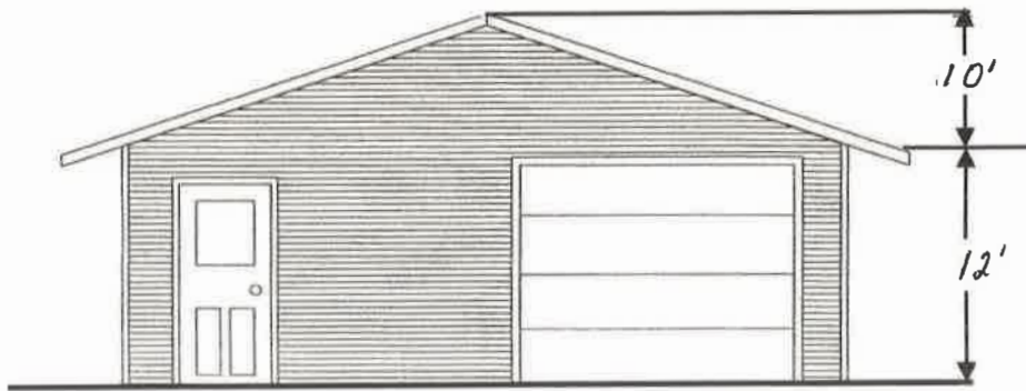
Front Elevation \frac{1}{4}'' = 1'
